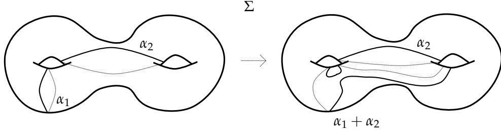
Figure 4.2: The curve \alpha_1 + \alpha_2 is the handleslide of \alpha_1 over \alpha_2 .
