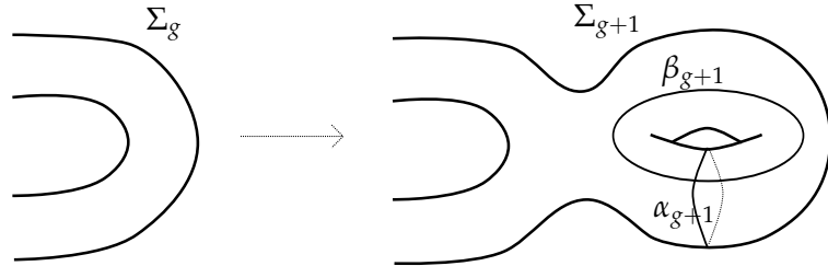
Figure 4.3: The new curves \alpha_{g+1} and \beta_{g+1} are in standard position. This move corresponds to a connected sum with S^3 .
