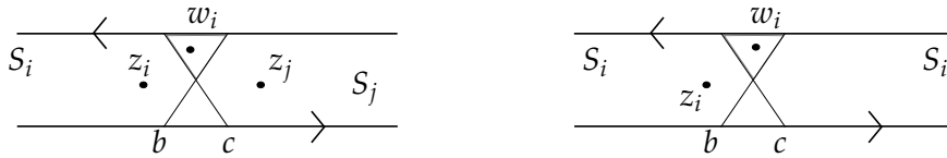
Figure 4.9: On the left S_i and S_j are different components of S \setminus \cup \mathcal{A}_i .
