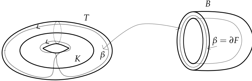
Figure 2.1: The ball B is attached to the solid torus T along the curve \beta .
