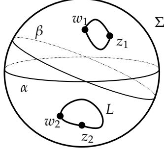
Figure 4.4: A very simple multi-pointed Heegaard diagram for the 2-component unlink in S^3 .
