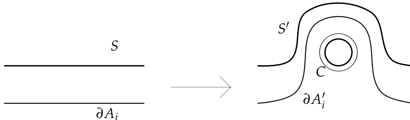
Figure 6.3: Abstract picture of the stabilization on S .
