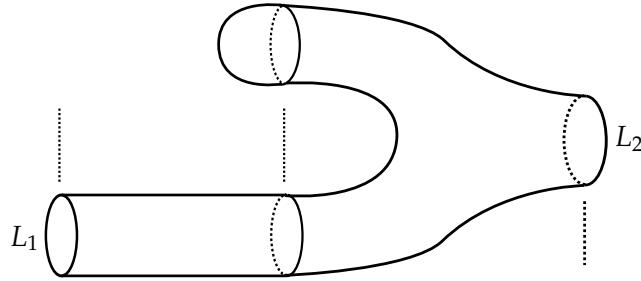
Figure 8.8: A more useful birth cobordism.
