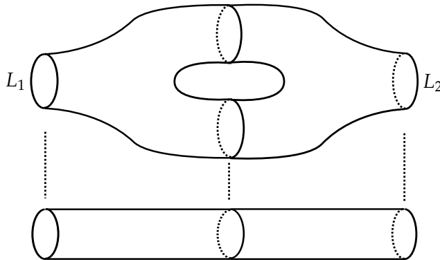
Figure 8.6: Torus cobordism.
