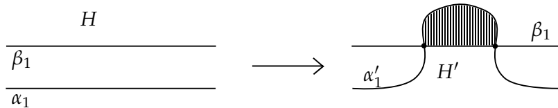
Figure 5.3: By moving the curve \alpha_1 to \alpha'_1 through a Hamiltonian isotopy, we introduce a pair of canceling intersection points.
