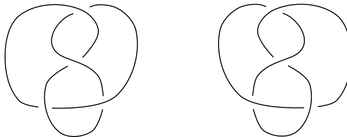
Figure 1.9: A diagram for the Figure-eight knot and its mirror image. It is easy to see that the two knots are isotopic.
